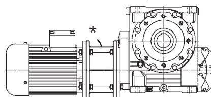
MLS / MLA montaggio tra riduttore e motore o motor-variator mounted between gear reducer and motor or motor-variator
